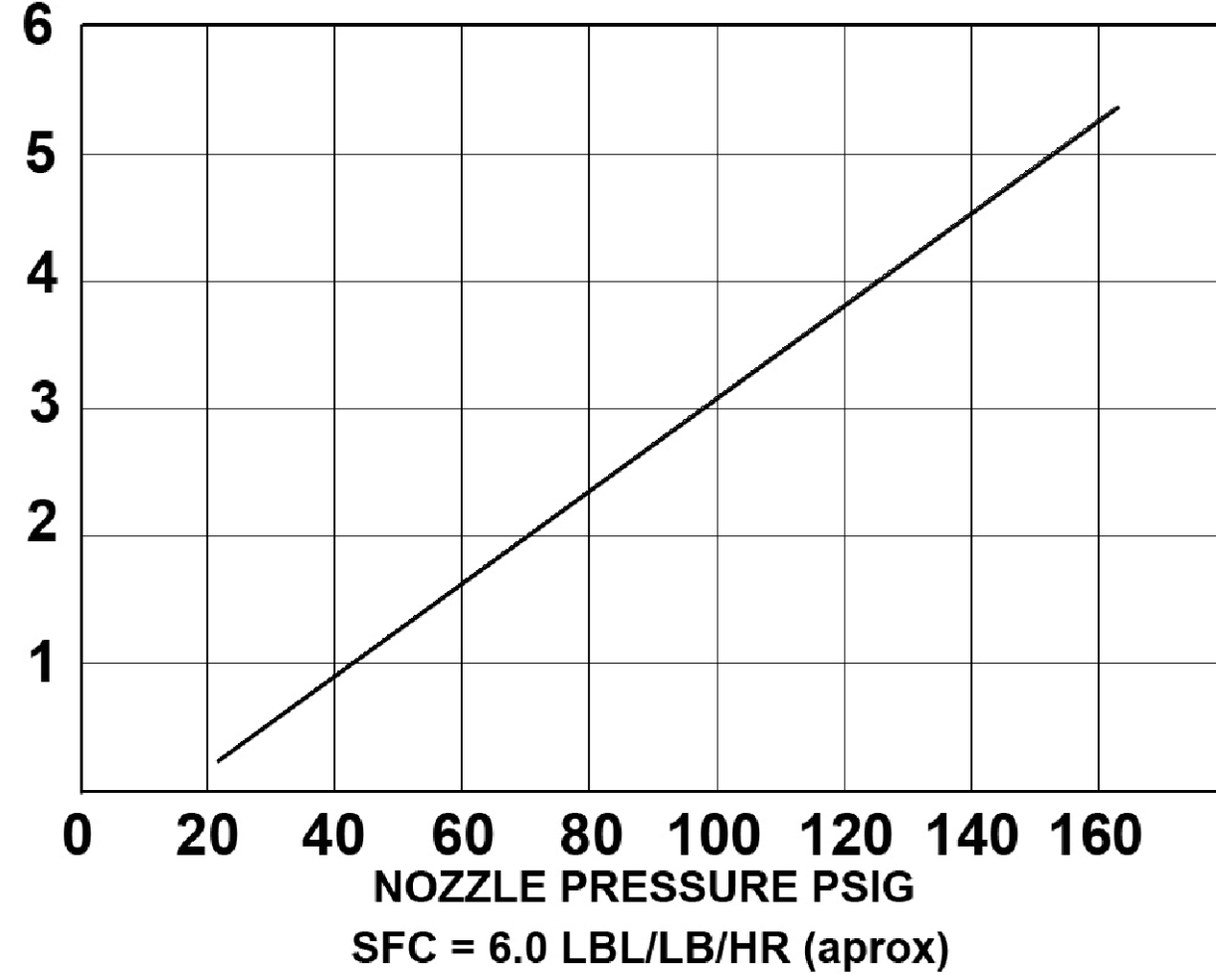
G8-2-5 JET STATIC PERFORMANCE
